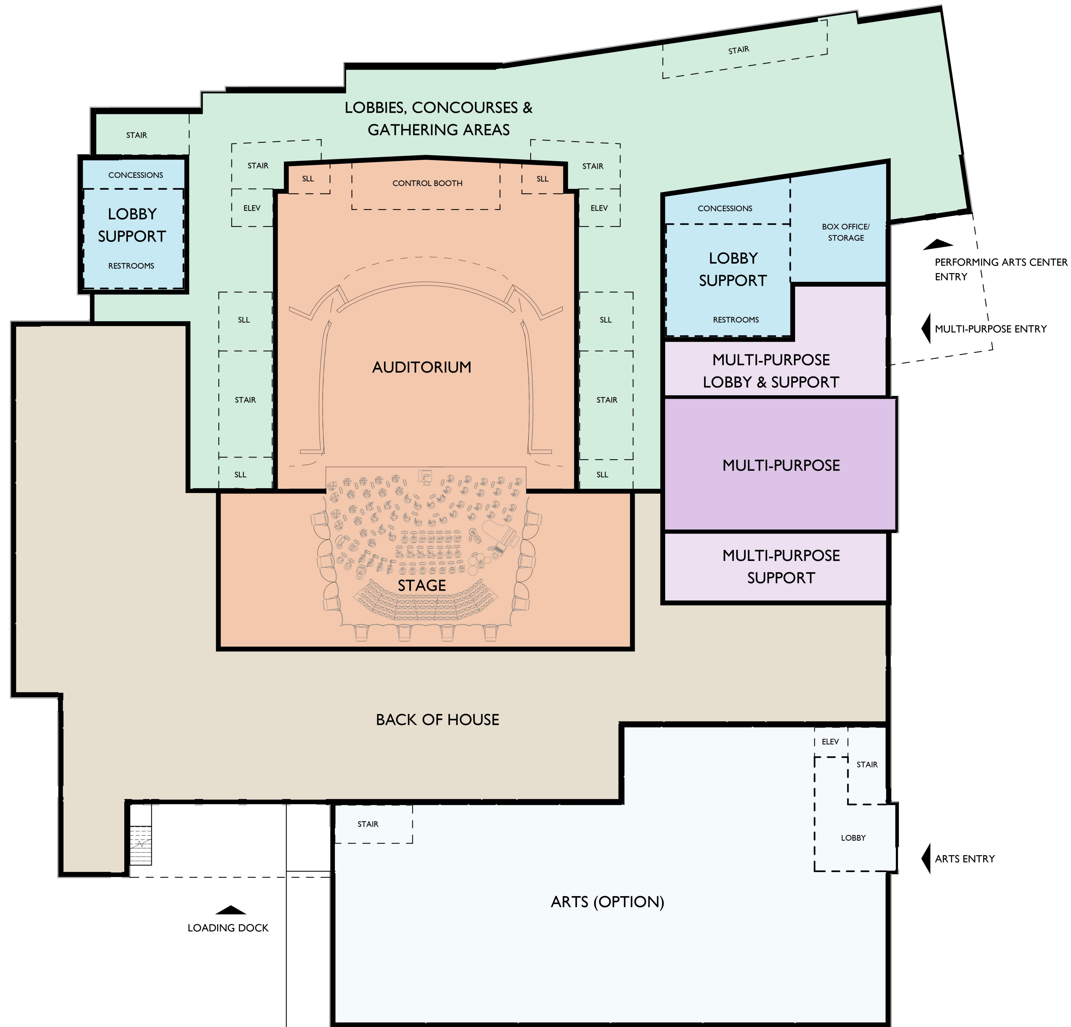
LEVEL 1 FLOOR PLAN
